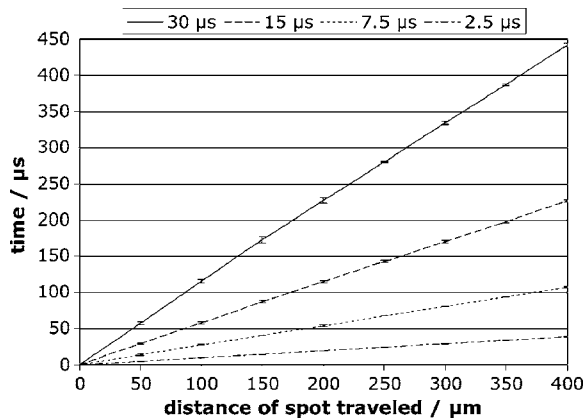
Fig. 5 Demonstration of the scan speed along the line being constant using our AOD. The data shown represent the measurements for 30-, 15-, 7.5-, and 2.5- \mu\text{s} exposures. In this work, the speed is always expressed in terms of its resulting exposure time, that is, the time the spot needs to travel a distance equivalent to its 1/e^2 diameter.
