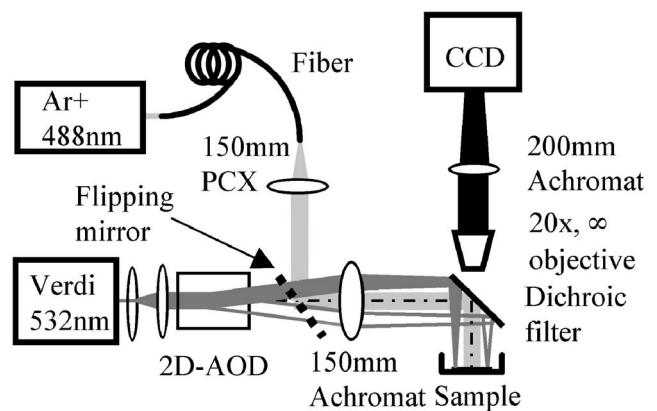
Fig. 3 Schematic of the bench-top in vitro setup. The output beam of the diode-pumped solid-state Verdi (5 mm) was enlarged to the size of the full active aperture of the 2-DAOD (5 mm) with a Keplerian beam expander. After passing the focusing achromat ( f.l.=150 mm) at the output side of the AOD, the first-order beam was directed vertically by a dichroic filter onto the sample, which was placed horizontally on a 3-D translation stage. A compound fluorescence microscope employing an infinity-corrected 20\times objective with a large working distance was erected on top of the dichroic filter and the sample holder to visualize the sample through a CCD camera. A fiber-coupled white light source illuminated the sample (not shown). Radiation from an argon ion laser (488 nm) was coupled into a multimode fiber. The fiber output was introduced into the beam path by a flipping mirror for fluorescence excitation of the viability assay Calcein.
