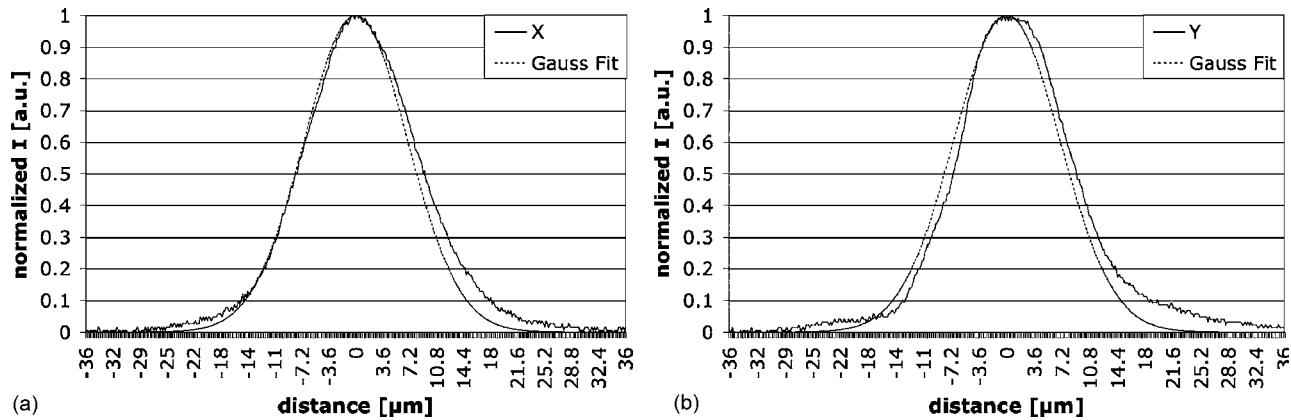
Fig. 8 Beam profile in air along (a) x and perpendicular (b) y to the direction of motion of the spot in the focal plane. The beam is 27.5 \mu\text{m} in diameter with a nearly Gaussian irradiance profile. Ratio of the measured spot diameter ( 1/e^2 ) of 27.5 \mu\text{m} over a calculated diffraction-limited diameter of 19.2 \mu\text{m} indicates M^2 of 1.4.
