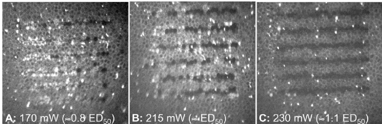
Fig. 6 Calcein fluorescence images after irradiation with 3 \mu\text{s} (all 10 repetitions with 100 Hz). Power increases from (a) to (c). Below ED_{50} , (a) few exposed cells are damaged. At about ED_{50} , (b) lines of dead cells are one or two cells wide; not all cells are damaged. Above ED_{50} , (c) all exposed cells were damaged and widening of the lines was observed. Clearly separated lines of dead cells, resembling the applied scan pattern, suggest selectivity of the method within the RPE monolayer.
