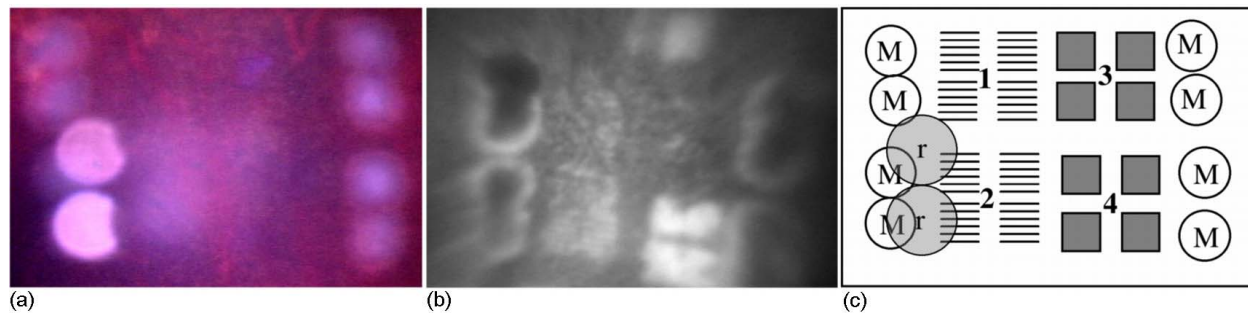
Fig. 10 View through the slit lamp (a) minutes after irradiation and corresponding fluorescence angiographic image (b) taken 1 h after irradiation of the same site with (c) additional corresponding sketch of the site. Selective lesions were placed between marker lesions (M), in which photoreceptors have been purposely coagulated by applying a very slow scan speed. Selective 7.5- \mu s exposures using separate lines were performed at (1) 1 \times ED_{50} and (2) 2 \times ED_{50} , and with interlaced lines also at (3) 1 ED_{50} and (4) 2 times ED_{50} . (a) All selective lesions were ophthalmoscopically invisible minutes post irradiation—the view in the lower left side of the image is partially obstructed by reflections (r) of the double-slit illumination from the contact lens. (b) Selective lesions become visible in fluorescence angiography as separated hyperfluorescent lines, where irradiation had been performed with the SEP scan pattern. Lesions close to the right column of markers were produced using the INT scan pattern; consequently, no separate fluorescence is visible.
