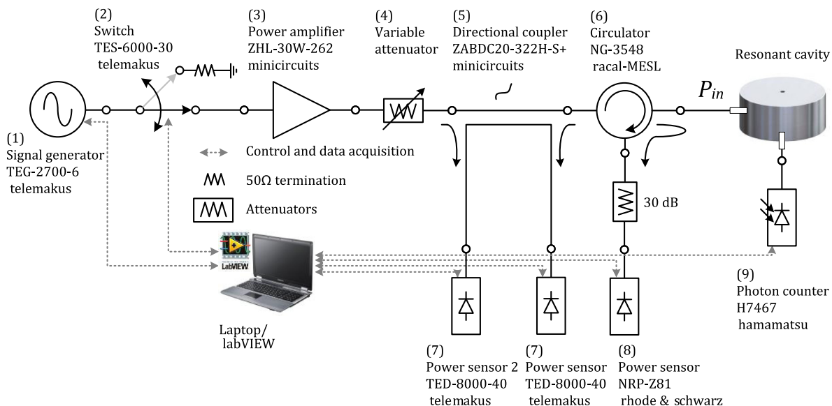
Fig. 2 Microwave circuitry and control system.
