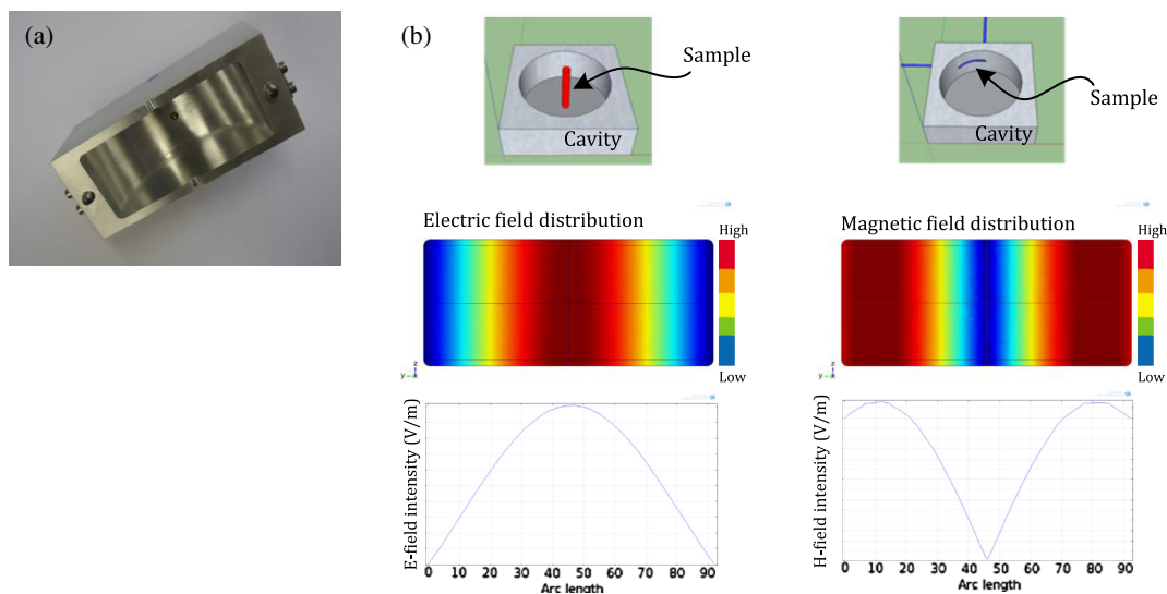
Fig. 1 (a) Inside view of the TM_{010} mode aluminum resonant cavity. (b) Three-dimensional representation of the electric (E) and magnetic (H) field set up, with sample tube placed axially or circumferentially, respectively. E- and H-field intensity plots are also shown.
