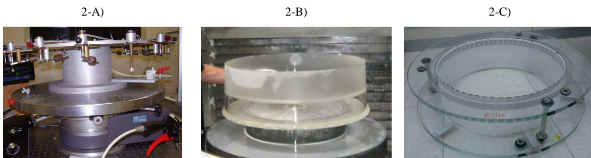
Fig. 2. A) Side view of the astatic support system used during OOR metrology. B) Raw quartz glass tube mounted on the grinding machine at the Heraeus Quarzglas facility. C) First shell integrated in its SSS.
