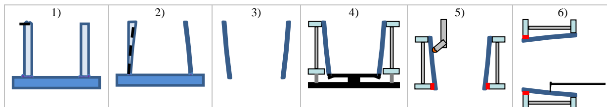
Fig. 1 Scheme of the production method under development for the manufacturing of thin quartz shells based on the direct figuring and polishing. 1) The raw starting material is a quartz glass tube, already available on the market; 2) The tube is positioned onto a suitable support and firstly ground to the required double-cone profile; 3) When the shell is ready, it is detached from the support; 4) By means of an astatic jig, it is measured and integrated in a support structure; 5-6) The jig allows the positioning of the shell in both vertical and horizontal positions whit respect to the optical axis without introducing deformations.
