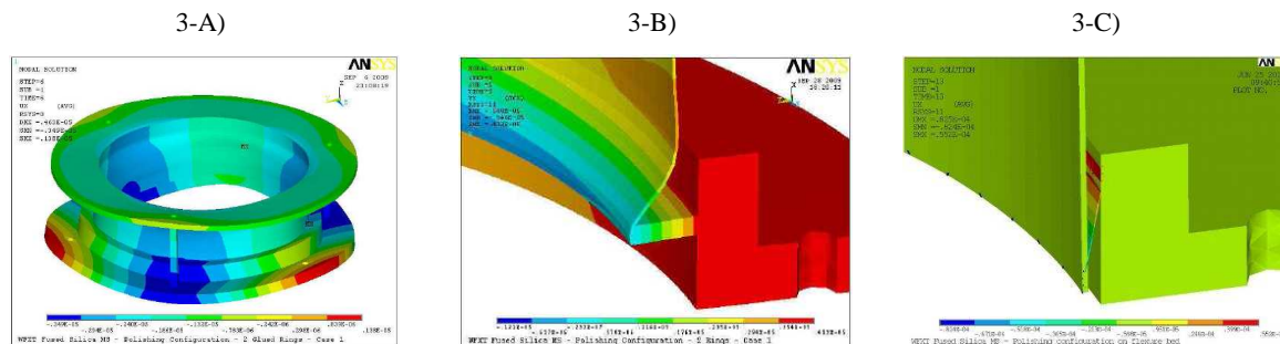
Fig. 3. A) FEM simulation carried out to verify the effect on the shell due to SSS deformations in the case of direct connection between the shell and the SSS. Deformations of the SSS are transmitted to the shell. B) Detail of radial displacement isocontours at the connection between the mirror shells and the SSS ring. The effect of the adhesive expansion due to thermal effects is evident. C) The use of a metal foil introduces a radial flexure, implemented in order to avoid the transmission of possible thermo-mechanical deformations into the shell.
