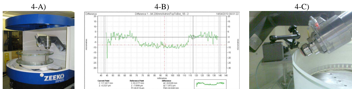
Fig. 4. A) Shell mounted on the Zeeko IRP600 machine. B) Example of the influence function of the grolishing process. The circle indicates the grolishing starting point. C) Particular of the Bonnet polishing tool during one of the first grolishing tests to evaluate the suitability of the SSS as interface to the polishing machine.
