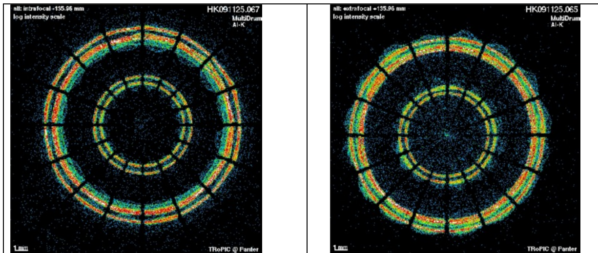
Fig. 15. Intra-focus image of the Test MM at 1.5keV
