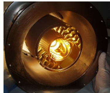
Fig. 10. Prototype Mirror Module integrated
