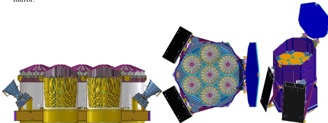
Fig. 1. eROSITA mirror modules configuration
