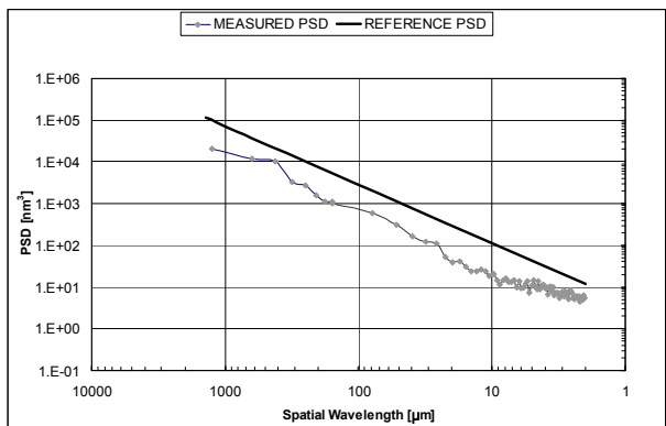
Fig. 3. One-dimensional PSDs compared with eROSITA reference PSD
