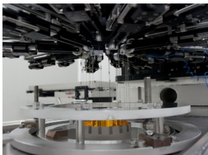
Fig. 8. Measurement of single shell performances on AVOB
