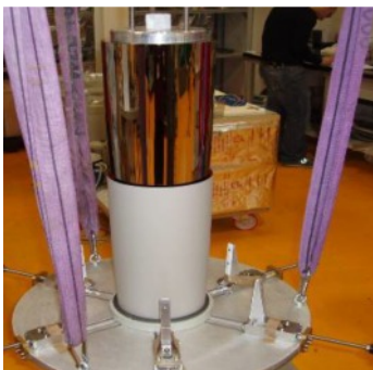
Fig. 5. Shell Release
