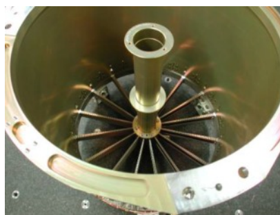
Fig. 12. Blocking shell and Mirror Interface Structure mounted on spider
