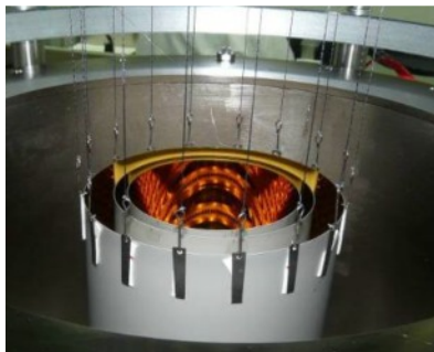
Fig. 9. Integration of Mirror Module with AVOB
