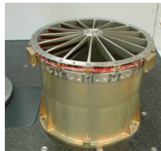
Fig. 13. Mirror module ready for shells integration
