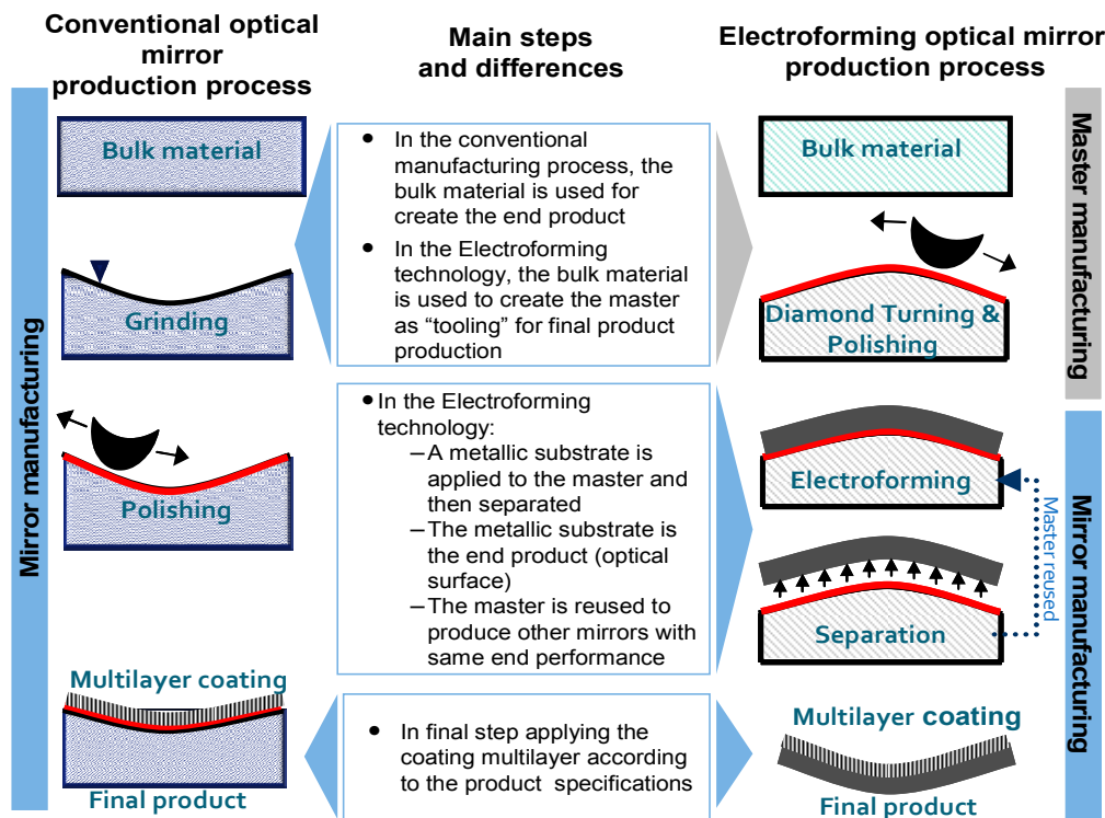
Fig. 2. Electroforming process
