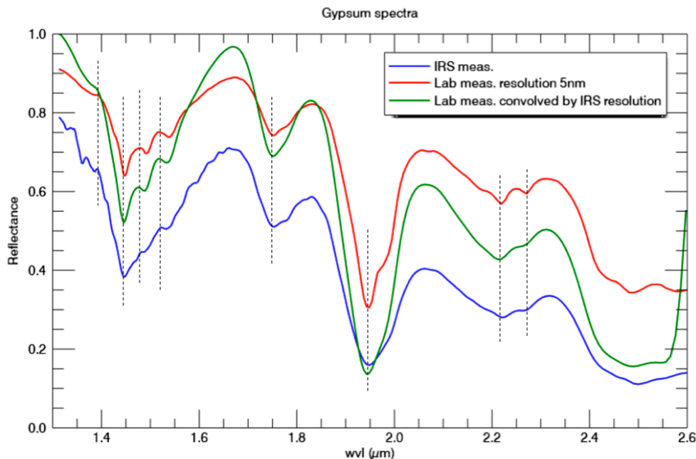
Figure 11: Comparison of gypsum reflectance measured with the IRS and with a lab spectrometer.
