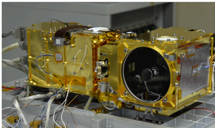
Figure 2: SCMU, EQM model
