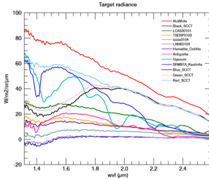
Figure 5: IR spectra of lab targets measured with the EQM
