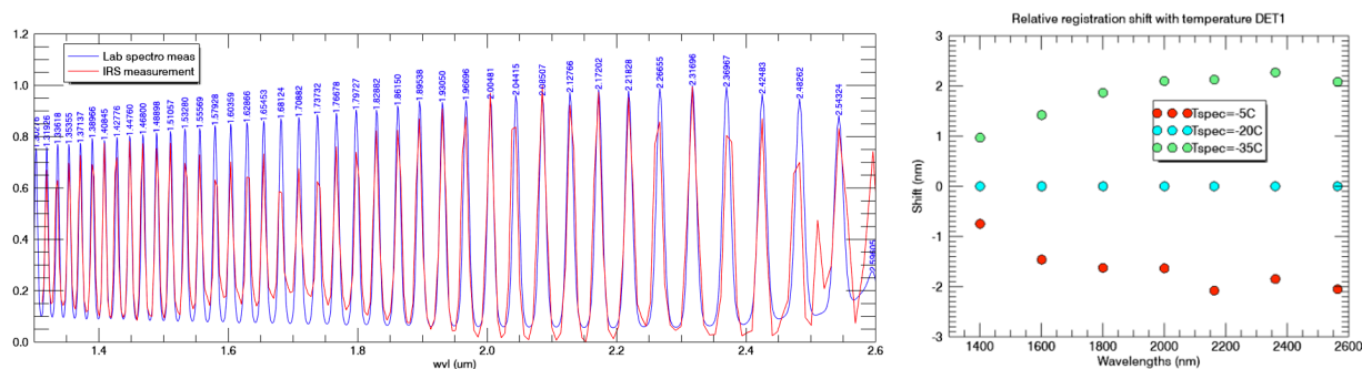
Figure 9: Fabry-Perot measurement with lab spectrometer and IRS (left) and relative spectral registration with spectrometer temperature (right).
