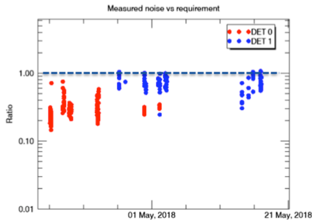
Figure 10: Noise for both photodiodes for all parameter conditions compared with the requirement
