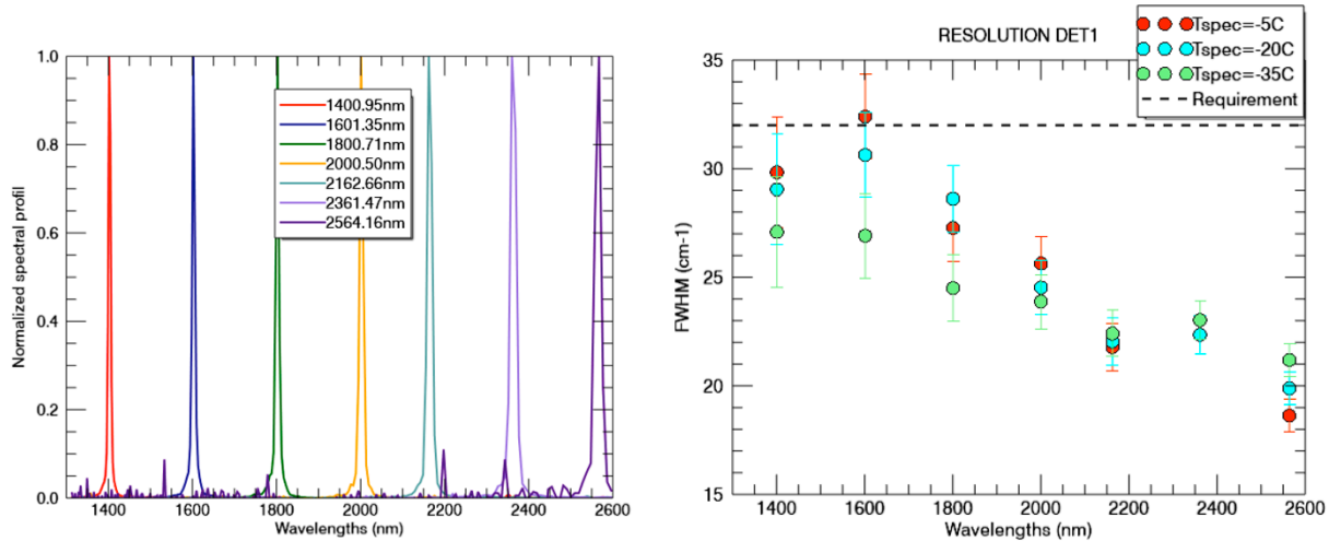
Figure 8: IRS response to different spectral stimuli by a monochromator (left) and calculated spectral resolution at different spectrometer temperatures (right)
