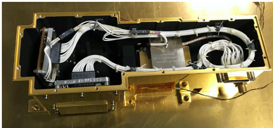
Figure 7: The Infrared spectrometer flight model. Total length = 173 mm.
