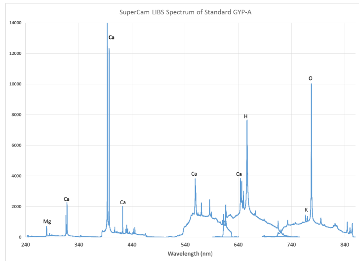
Figure 3: LIBS spectrum of GYP-A
