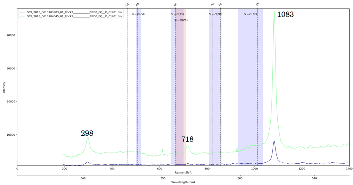
Figure 4: Raman spectrum of a rhodinite rock measured with the EQM
