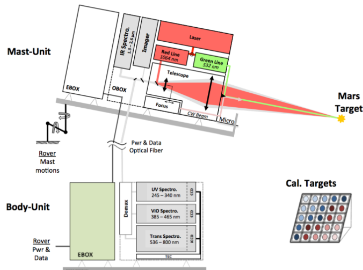
Figure 1: The SuperCam Instrument block diagram
