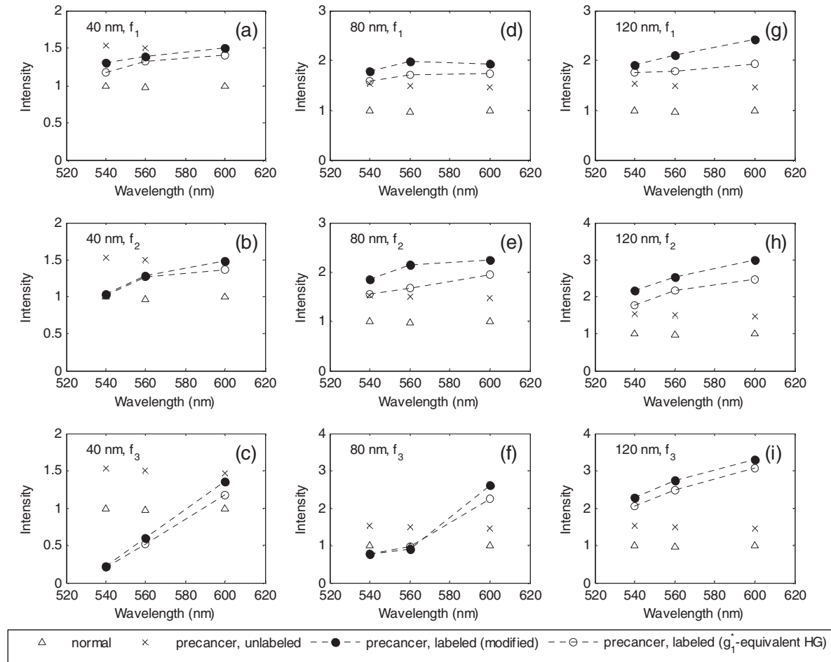
Fig. 7 Modeled reflectance response of normal tissue, unlabeled precancerous tissue, and precancerous tissue labeled with gold nanoparticles. Possible combinations of nanoparticle sizes (40, 80, and 120 nm) and volume fractions ( f_1 = 0.0005\% , f_2 = 0.001\% , and f_3 = 0.005\% ) result in nine different labeling schemes: (a) 40 nm; f_1 , (b) 40 nm; f_2 , (c) 40 nm; f_3 , (d) 80 nm; f_1 , (e) 80 nm; f_2 , (f) 80 nm; f_3 , (g) 120 nm; f_1 , (h) 120 nm; f_2 , and (i) 120 nm; f_3 . The distal ends of the source and detector fibers are tilted toward each other and are separated by a center-to-center distance of 300 \mu\text{m} .
