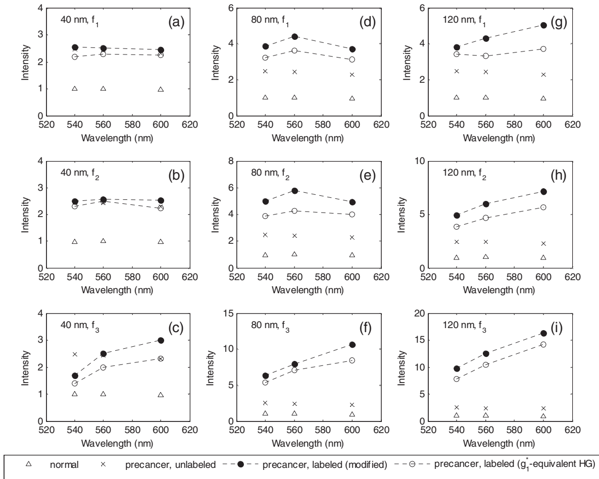
Fig. 6 Modeled reflectance response of normal tissue, unlabeled precancerous tissue, and precancerous tissue labeled with gold nanospheres. Possible combinations of nanoparticle sizes (40, 80, and 120 nm) and volume fractions ( f_1 = 0.0005\% , f_2 = 0.001\% , and f_3 = 0.005\% ) result in nine different labeling schemes: (a) 40 nm; f_1 , (b) 40 nm; f_2 , (c) 40 nm; f_3 , (d) 80 nm; f_1 , (e) 80 nm; f_2 , (f) 80 nm; f_3 , (g) 120 nm; f_1 , (h) 120 nm; f_2 , and (i) 120 nm; f_3 . The distal ends of the source and detector fibers are tilted toward each other and are separated by a center-to-center distance of 150 \mu\text{m} .
