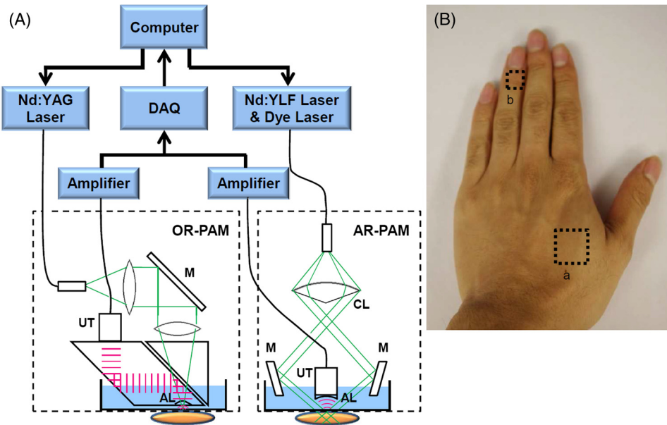
Fig. 1 (A) Schematic of the optical-resolution (OR-PAM) and acoustic-resolution photoacoustic microscopy (AR-PAM) systems. AL, acoustic lens; CL, conical lens; DAQ, data acquisition system; M, mirror; UT, ultrasound transducer. (B) Photograph of the hand, showing the scanned regions: (a) region scanned by AR-PAM and (b) region scanned by OR-PAM.
