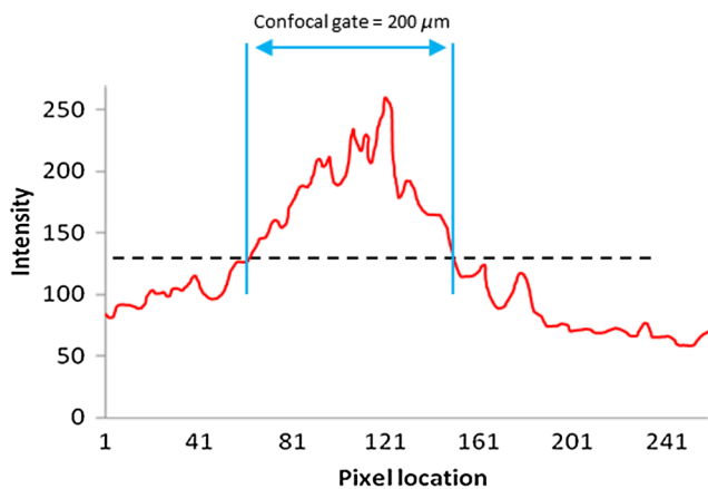
Fig. 16 Averaged smoothed A-line intensity profile of the image given in Fig. 15(e) (red rectangle). The confocal gate computed from the profile is 200 μm.
