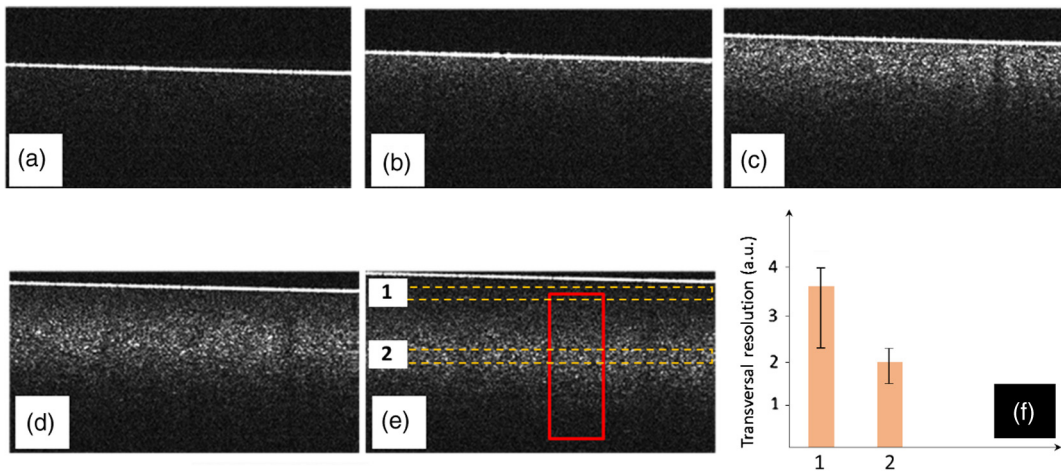
Fig. 15 SS-OCT B-scan images of a phantom composed of super white polyester microspheres embedded in epoxy-resin. Image size is 1.5 mm (lateral) × 2 mm (vertical, measured in air). OPD is zero. (a) Focus is on the surface of the sample, (b) focus is 200 μm inside the sample, (c) focus is 400 μm inside the sample, (d) focus is 600 μm inside the sample, (e) focus is 800 μm inside the sample, and (f) relative transversal resolution range along the rectangular areas 1 and 2 specified on (e). The rectangular areas 1 and 2 are the representative areas from which the transversal resolutions (in focus and out of focus) are calculated.
