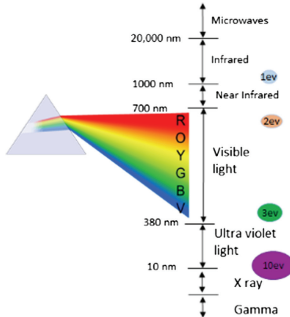
Figure 1.2 Electromagnetic spectrum.
