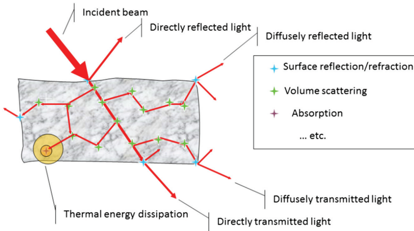
Figure 1.3 Laser–tissue interaction.
